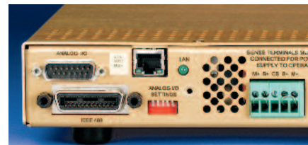
Rear view, Ethernet (LAN) port, E-Series Models
